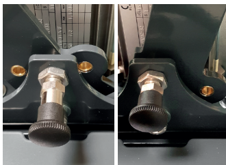
Locking with detent pins (special accessories)
